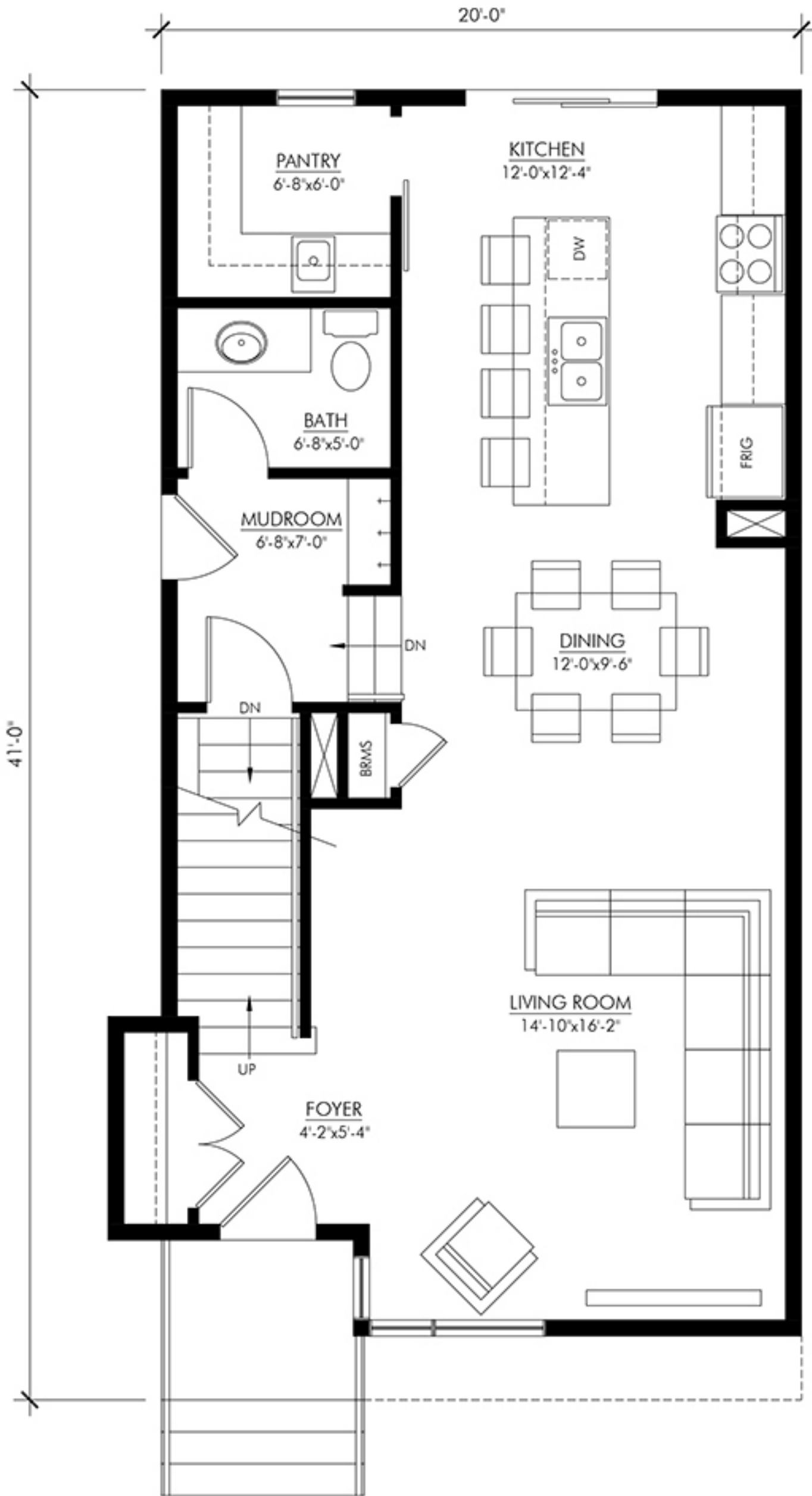
MAIN FLOOR PLAN - 774 SQ FT TWO STOREY - 1576
