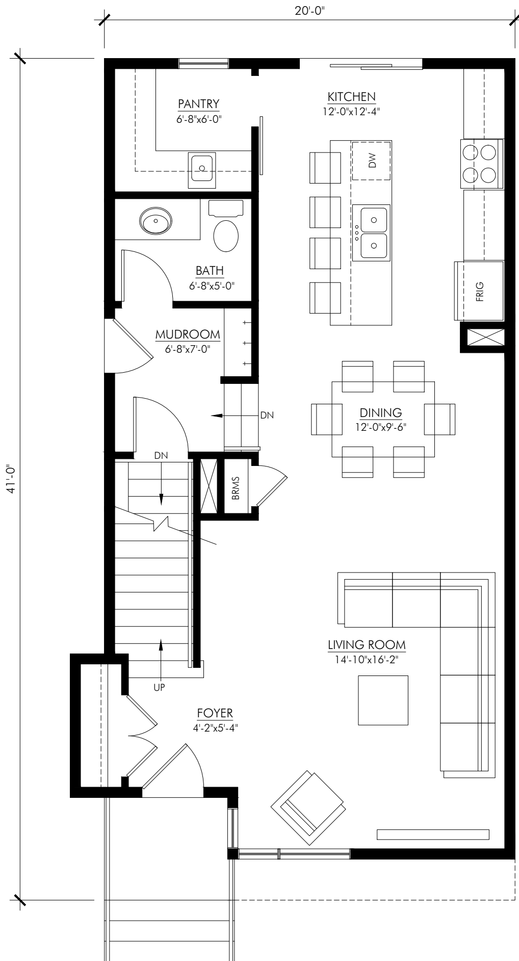
MAIN FLOOR PLAN - 774 SQ FT TWO STOREY - 1576
