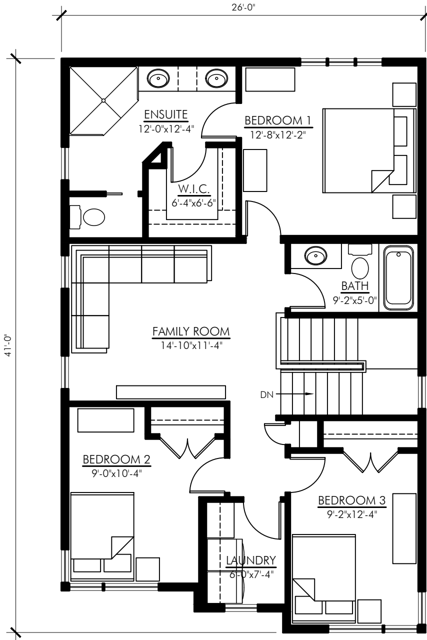
SECOND FLOOR PLAN - 1028 SQ FT BREMAN - 2007
