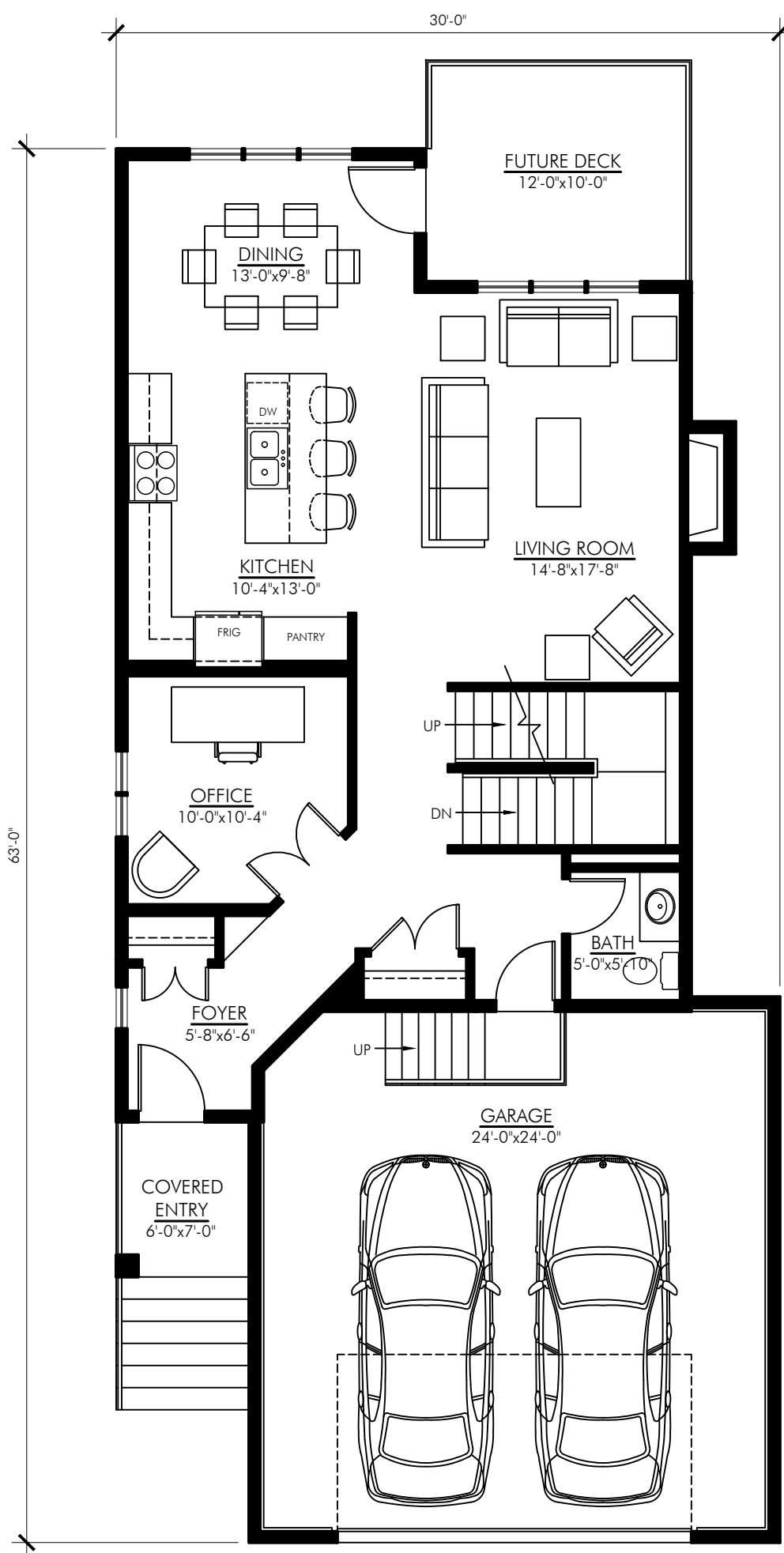
MAIN FLOOR PLAN - 979 SQ FT BREMAN - 2007
