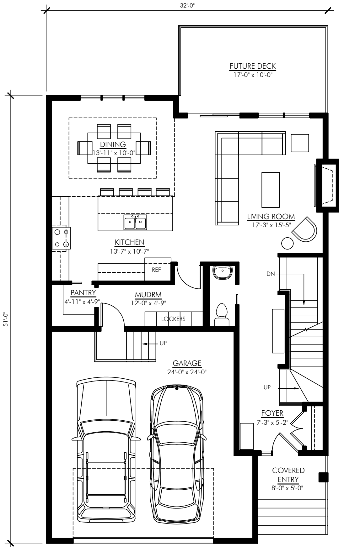
MAIN FLOOR PLAN - 976 SQ FT ATHENA - 2163
