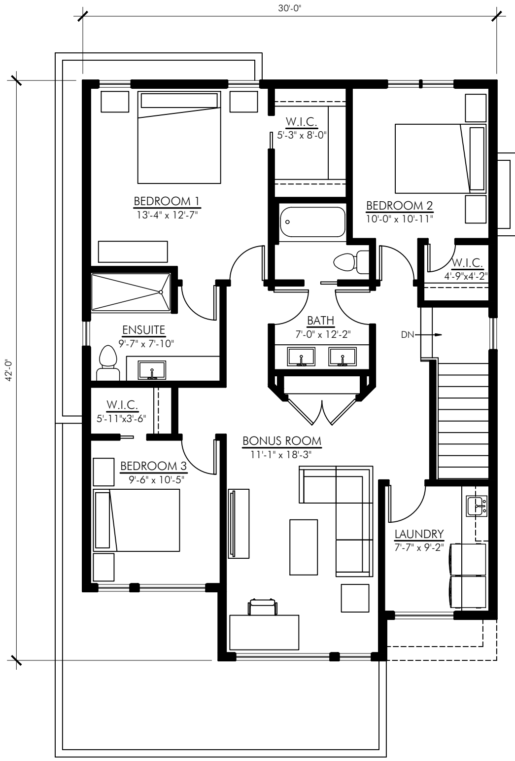
SECOND FLOOR PLAN - 1187 SQ FT ATHENA - 2163
