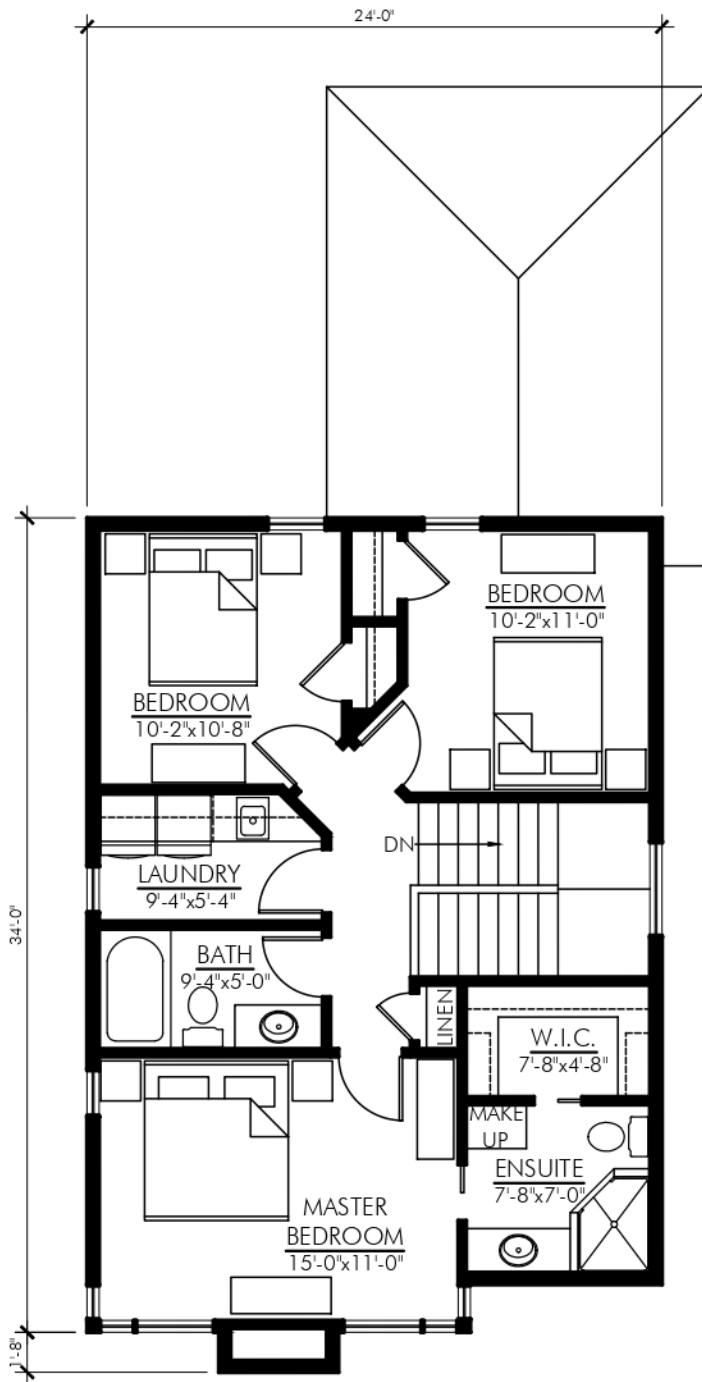
SECOND FLOOR PLAN - 800 SQ FT WATERBANK-1568
