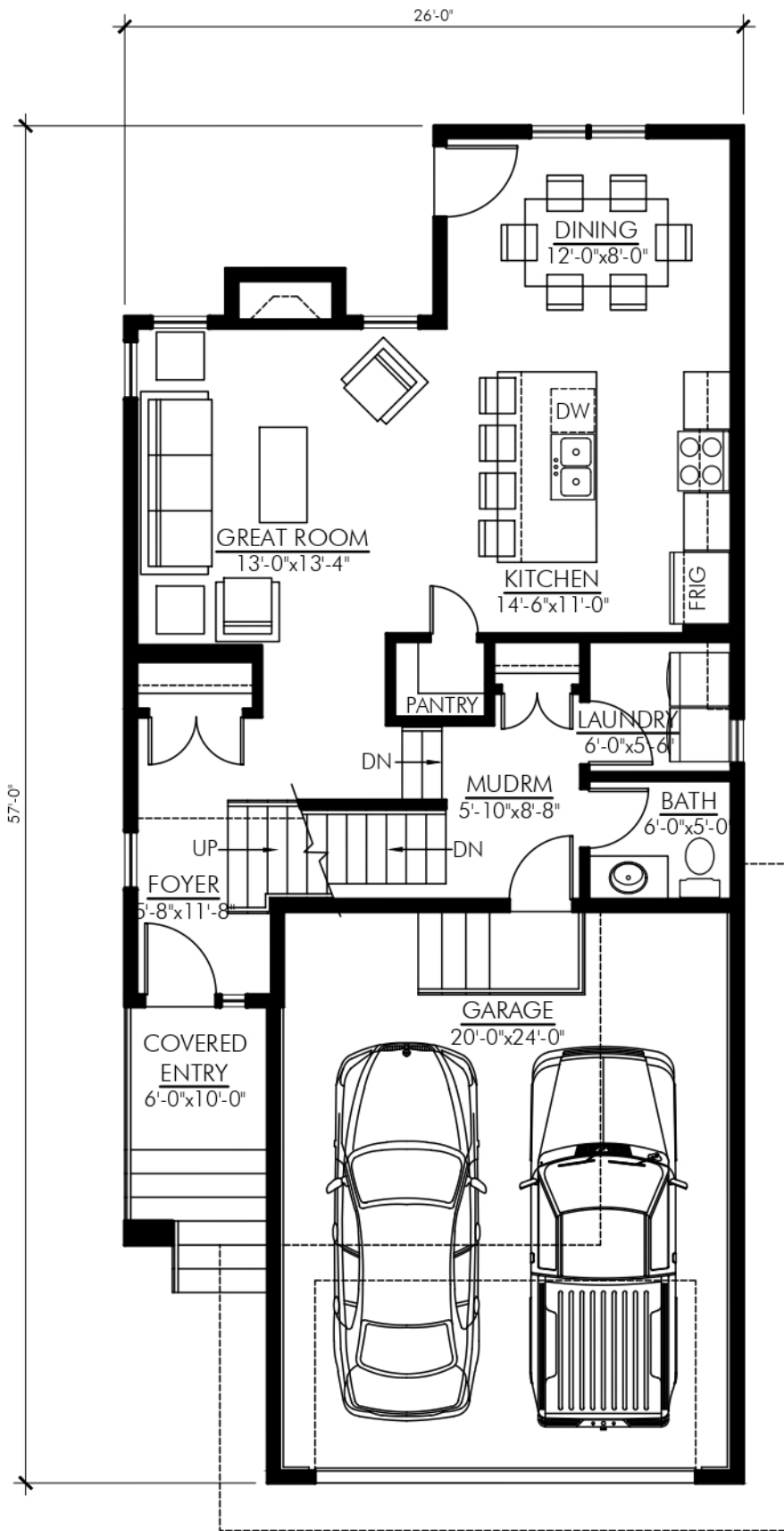
MAIN FLOOR PLAN - 781 SQ FT JASPER-1720
