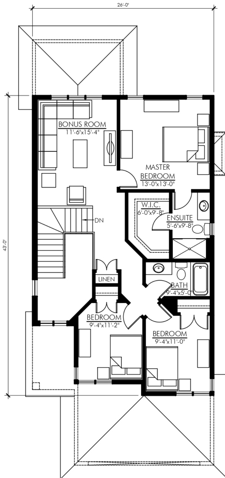
SECOND FLOOR PLAN - 965 SQ FT BRISTOL-1853
