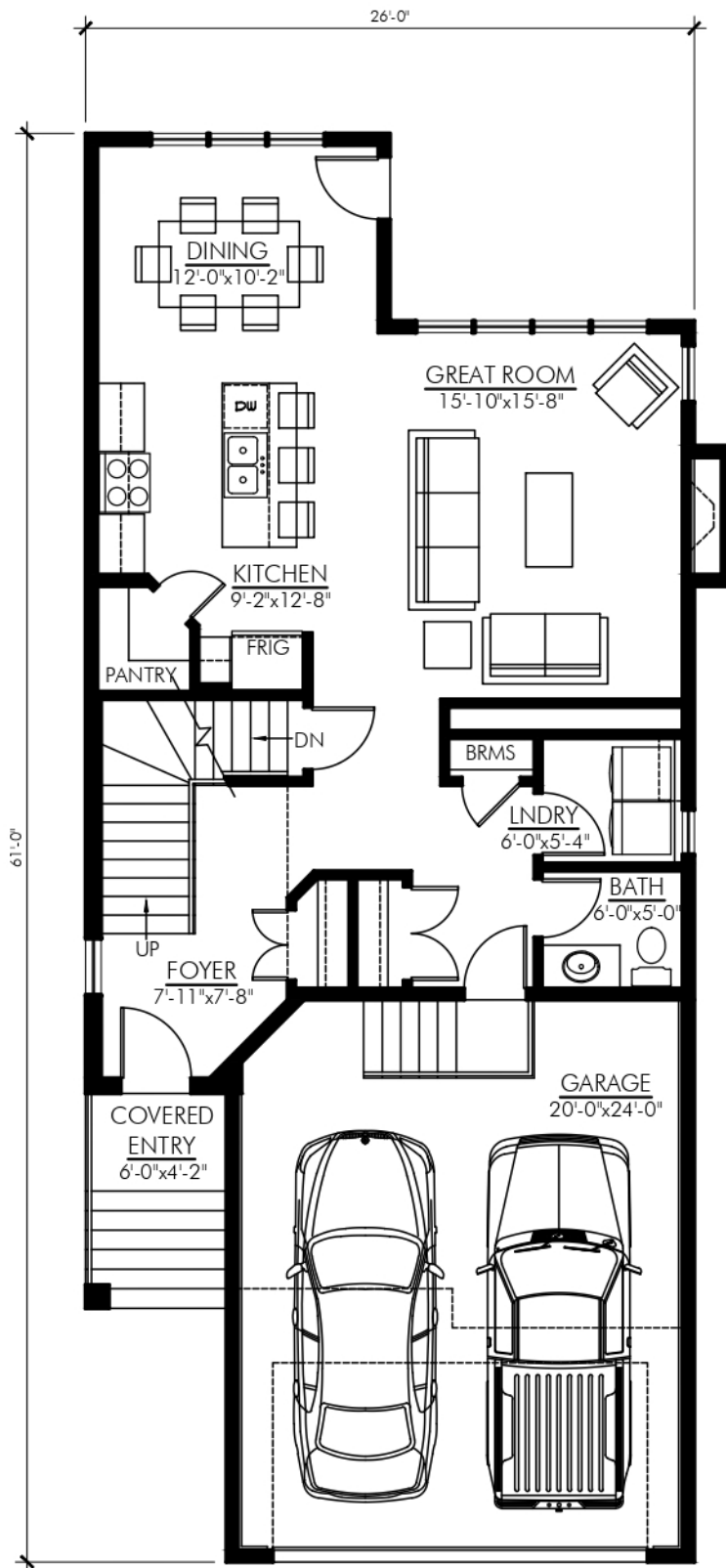
MAIN FLOOR PLAN - 888 SQ FT BRISTOL-1853
