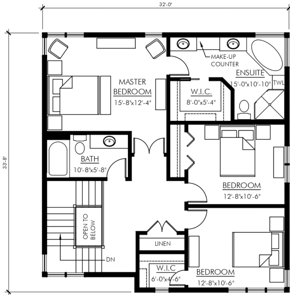
SECOND FLOOR PLAN - 1053 SQ FT THE ARCOLA - 2251
