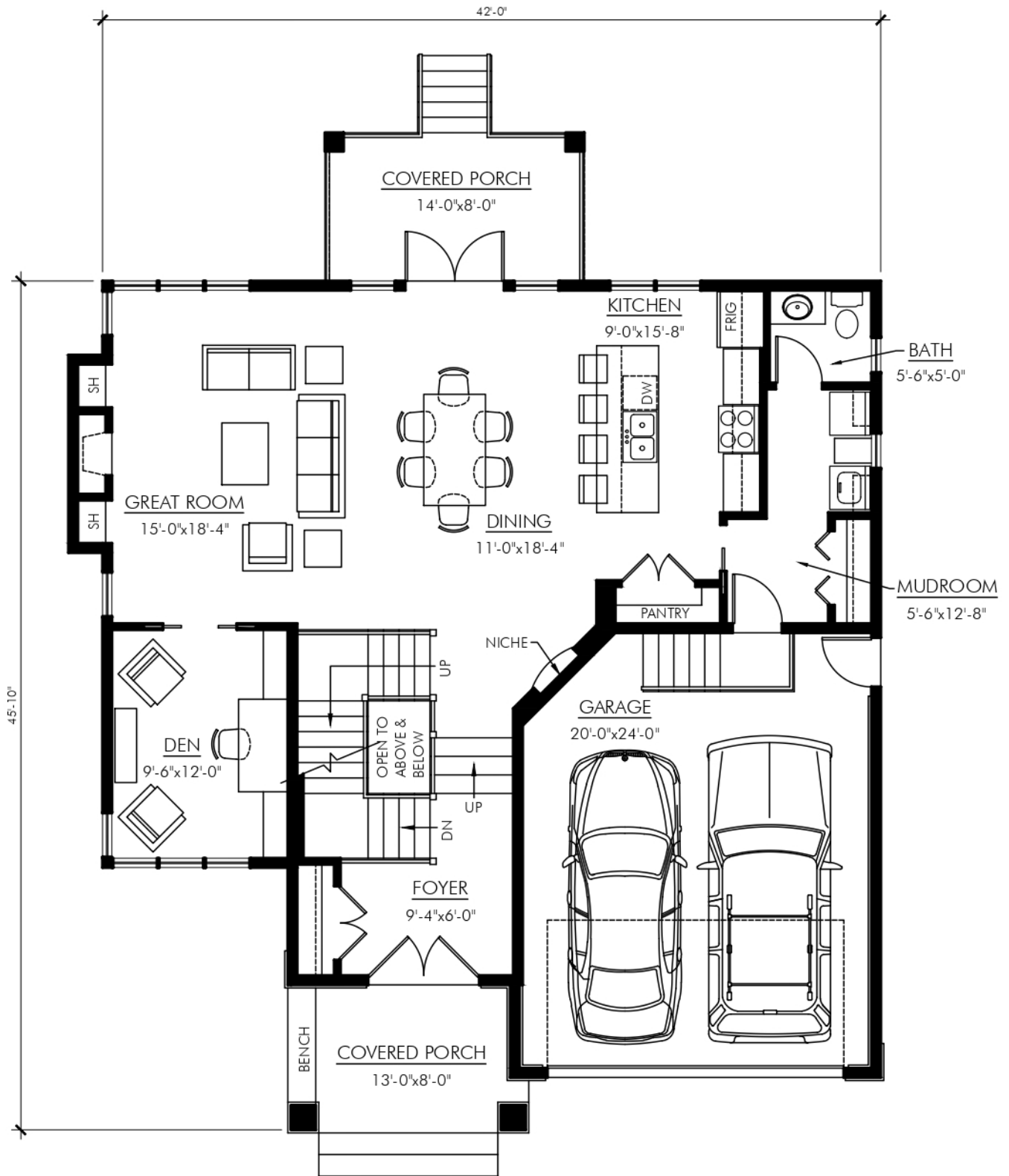
MAIN FLOOR PLAN - 1198 SQ FT THE ARCOLA - 2251
