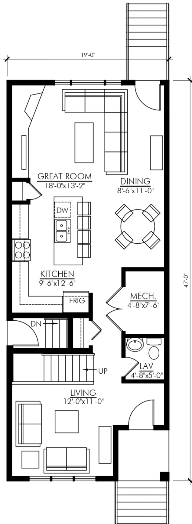
MAIN FLOOR PLAN - 857 SQ. FT. AQUILA-1714
